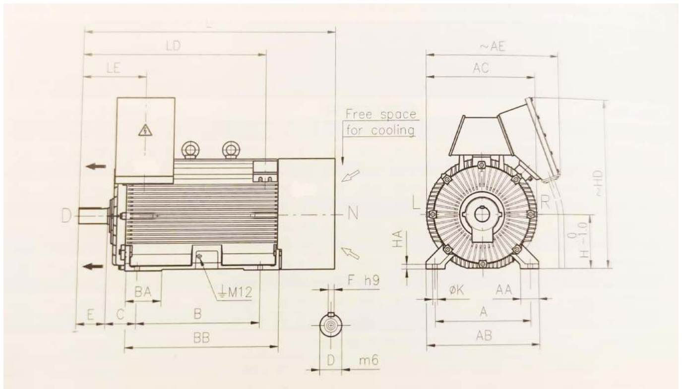
MOTOR DIMENSION DRAWING
